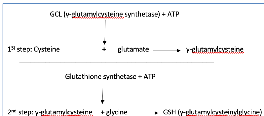
Figure 5 - The two steps synthesis of glutathione 5,11,20
